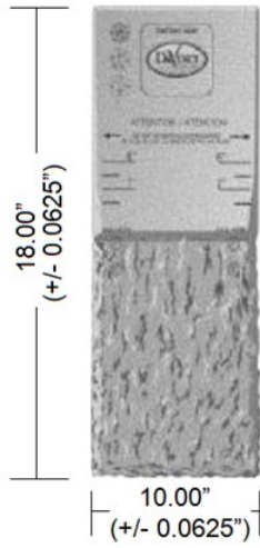
FIGURE 1—DaVINCI SLATE, DaVINCI SHAKE AND DaVINCI SELECT SHAKE SHAKE ROOF SHINGLES
