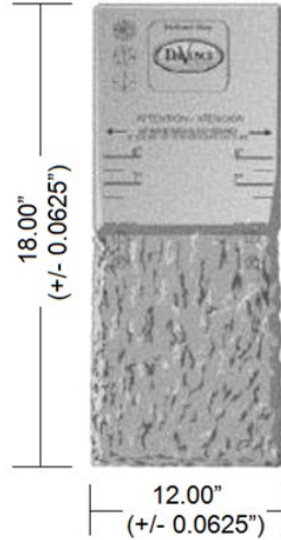
FIGURE 1—DaVINCI SLATE, DaVINCI SHAKE AND DaVINCI SELECT SHAKE SHAKE ROOF SHINGLES
